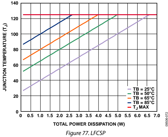
Figure 77. LFCSP
