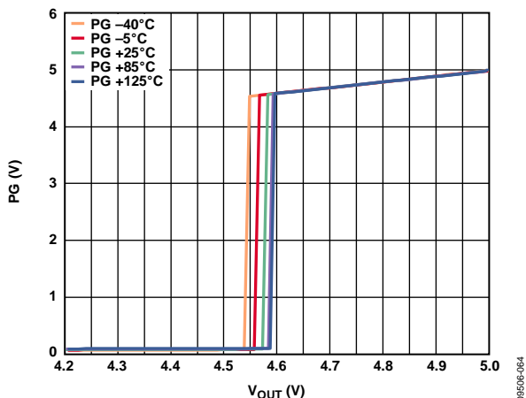
Figure 69. Typical Power Good Threshold vs. Temperature, VOUT Falling
