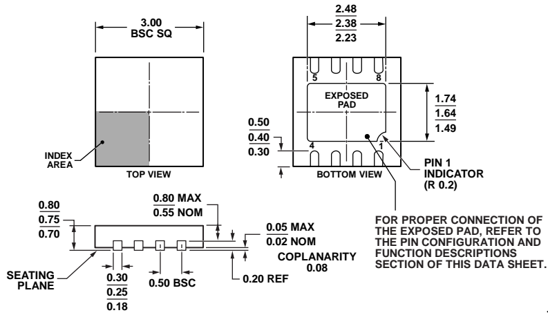
Figure 81. 8-Lead Lead Frame Chip Scale Package [LF CSP_WD] 3 mm x 3 mm Body, Very Very Thin, Dual Lead (CP-8-5) Dimensions shown in millimeters
