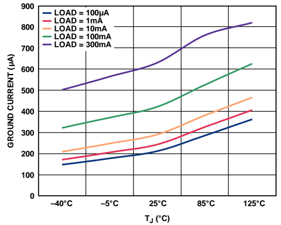
Figure 27. Ground Current vs. Junction Temperature, V_{OUT} = 1.8V
