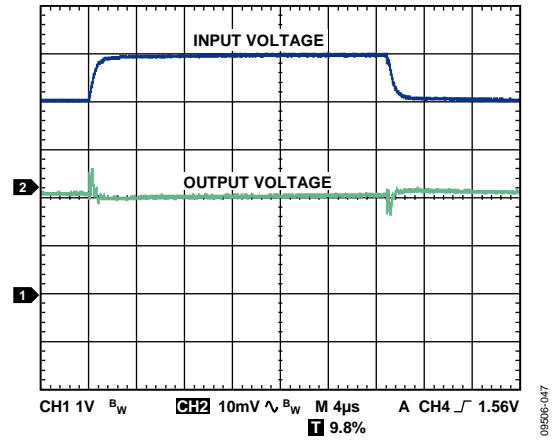
Figure 54. Line Transient Response, C_{IN}, C_{OUT} = 1 \mu F, I_{LOAD} = 300 \text{ mA}, V_{OUT} = 1.8 \text{ V}
